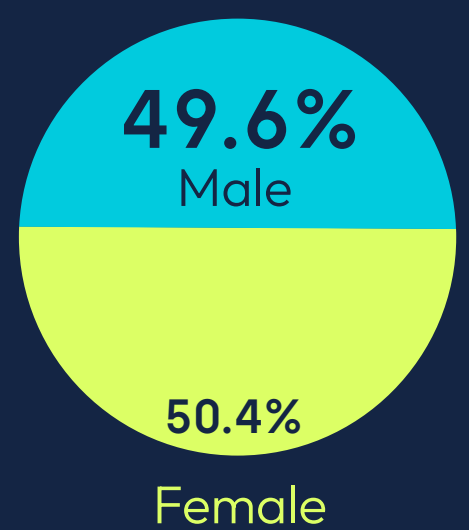
Lower quartile
