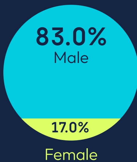
Upper quartile
